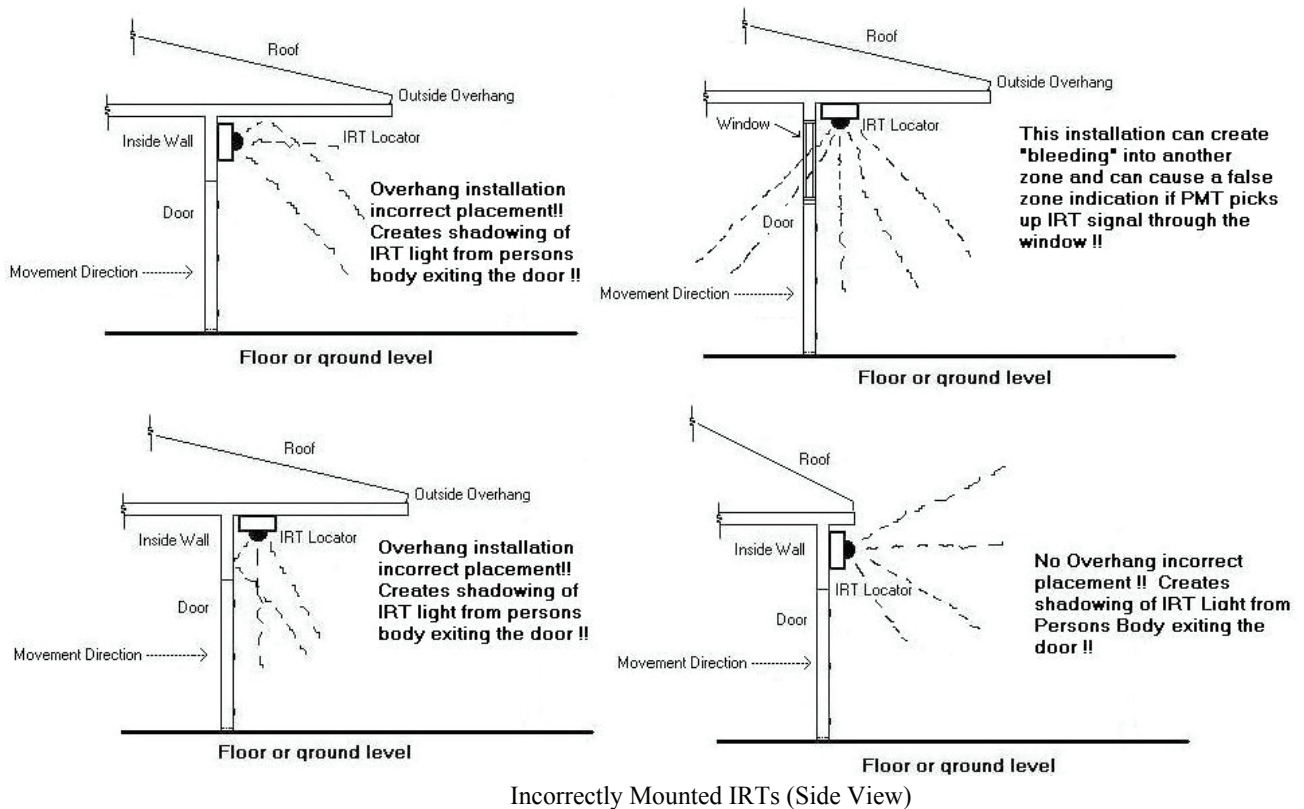
Incorrectly Mounted IRTs (Side View)
